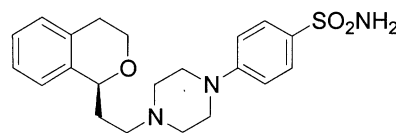
U-101387
