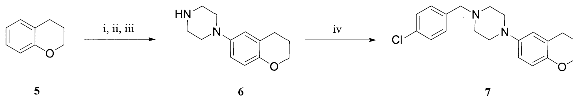
Scheme 2. Reaction conditions: (i) HNO 3 , 0 °C, 79%; (ii) Raney nickel, H 2 , 1 atm, 91%; (iii) bis-(2-chloroethyl)amine hydrochloride, K 2 CO 3 , chlorobenzene, reflux, 53%; (iv) 4-chlorobenzyl bromide, K 2 CO 3 , CH 3 CN, reflux, 79%.
