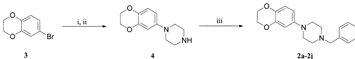
Scheme 1. Reaction conditions: (i) Pd 2 (dba) 3 , P(o-tolyl) 3 , tert -butyl 1-piperazinecarboxylate, NaO t Bu, PhMe, 100 °C, 55%; (ii) TFA, CH 2 Cl 2 , 20 °C, 82%; (iii) benzyl halide, K 2 CO 3 , CH 3 CN, reflux, 48–89%.
